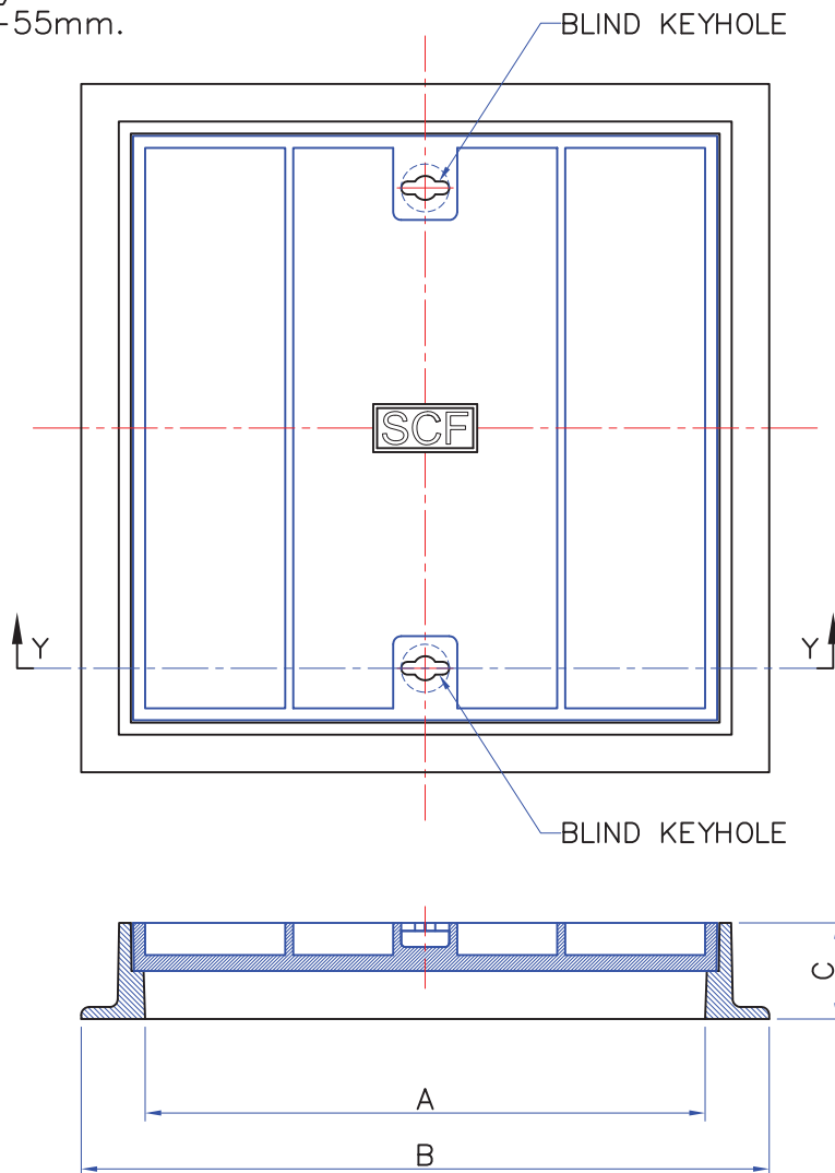
SECTION Y-Y
